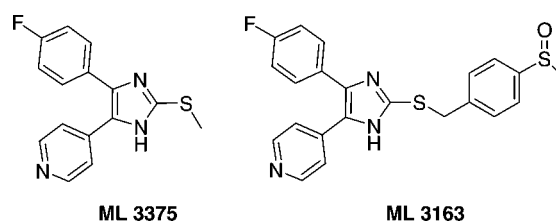
Figure 2. Pyridinyl imidazole inhibitors ML3163 and ML3375 of MERCKLE. 15
